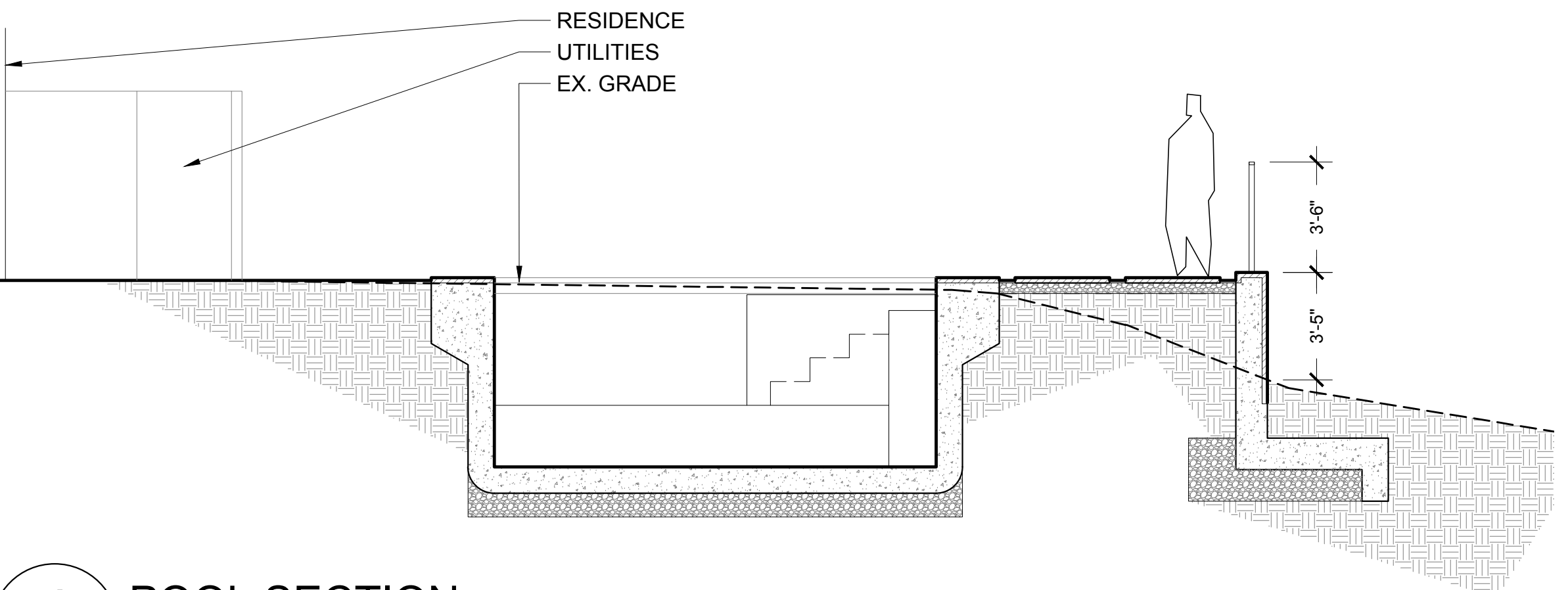
1 POOL SECTION SCALE: 1/4"=1'-0"
