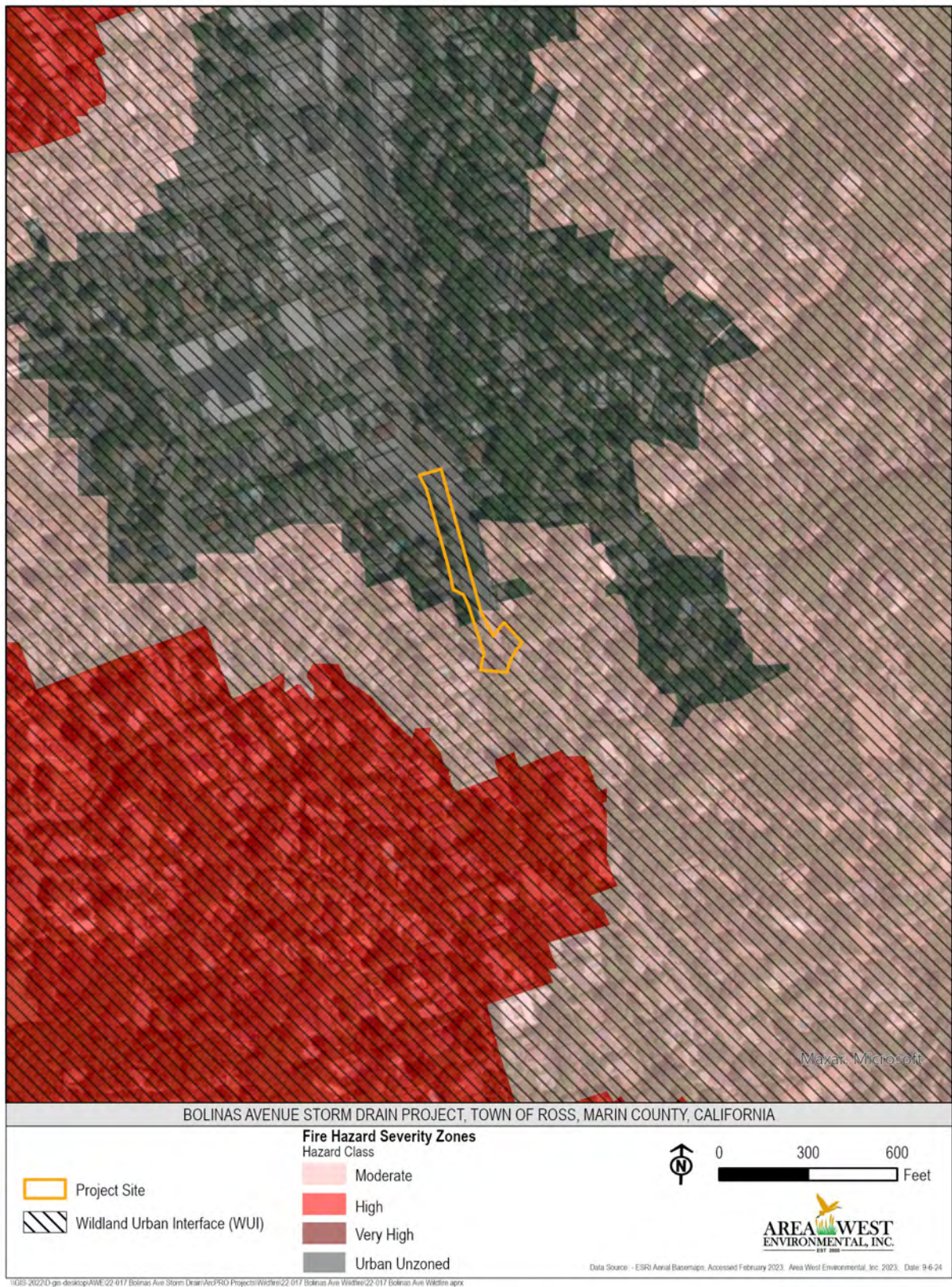
Figure 10. Fire Hazard Severity Level
