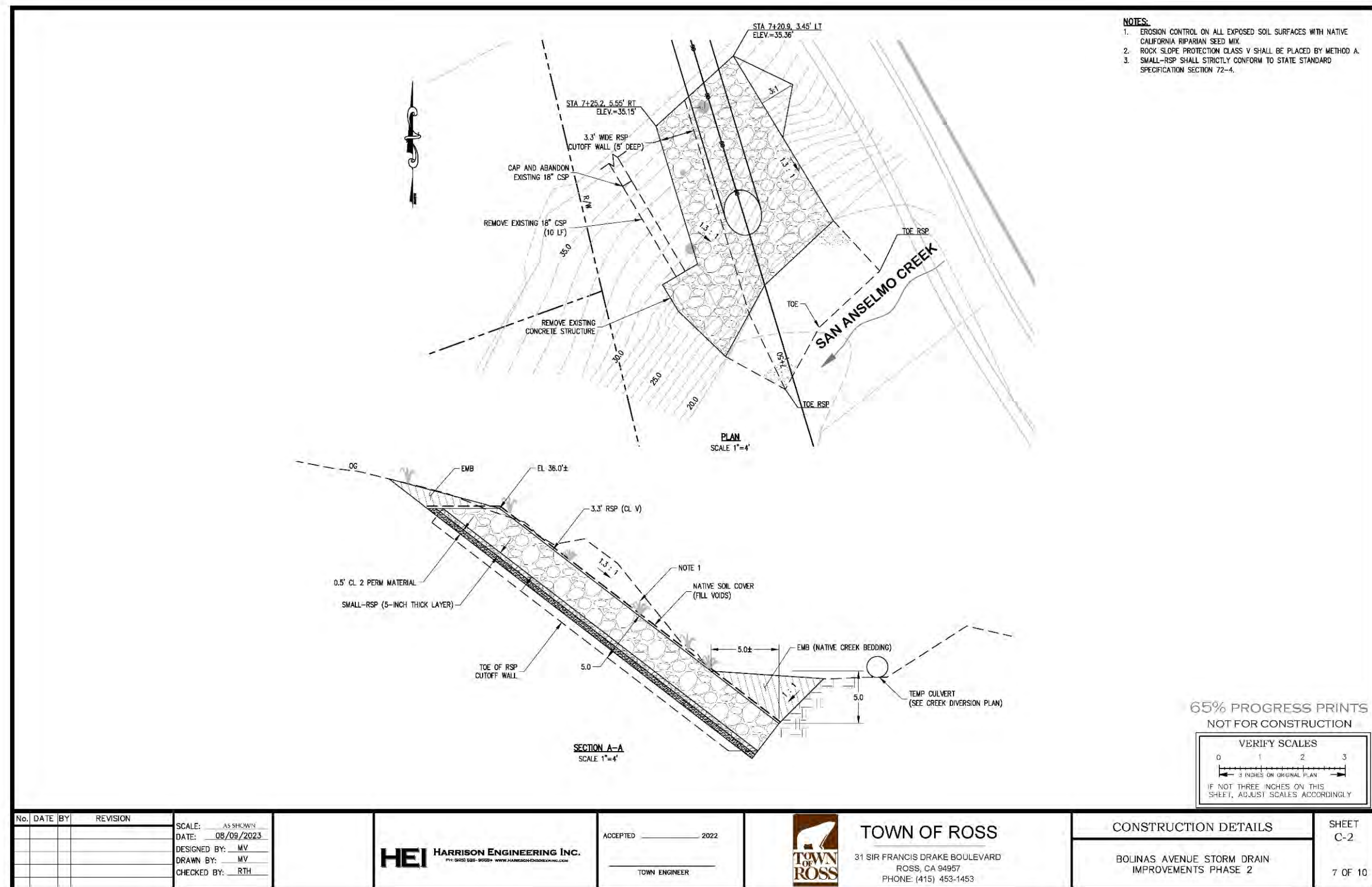
Figure 4. Outfall Design
